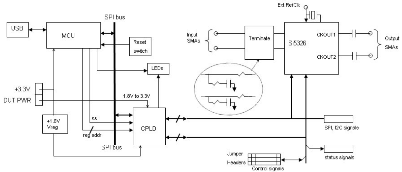
Figure 2. Si532x TQFP Block Diagram
