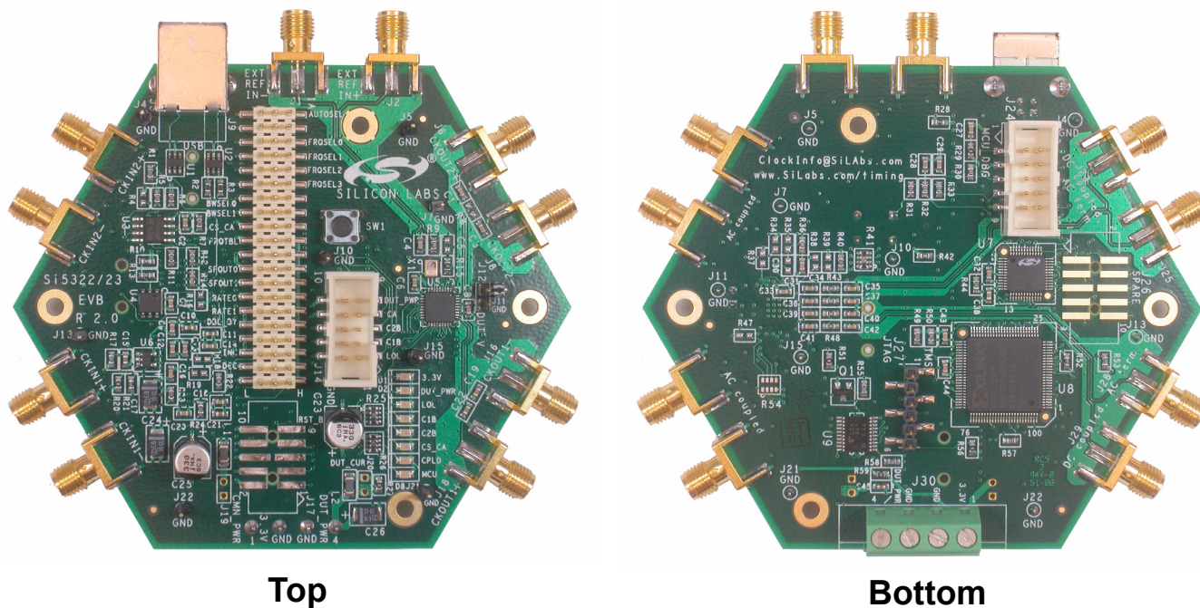
Figure 1. Si532x QFN EVB
